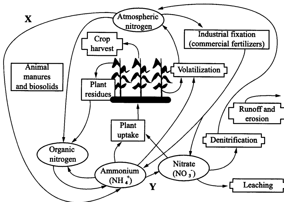
Figure 2. The nitrogen cycle
